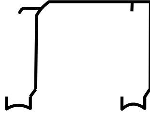
# 2200 ALUMINUM TRACK
