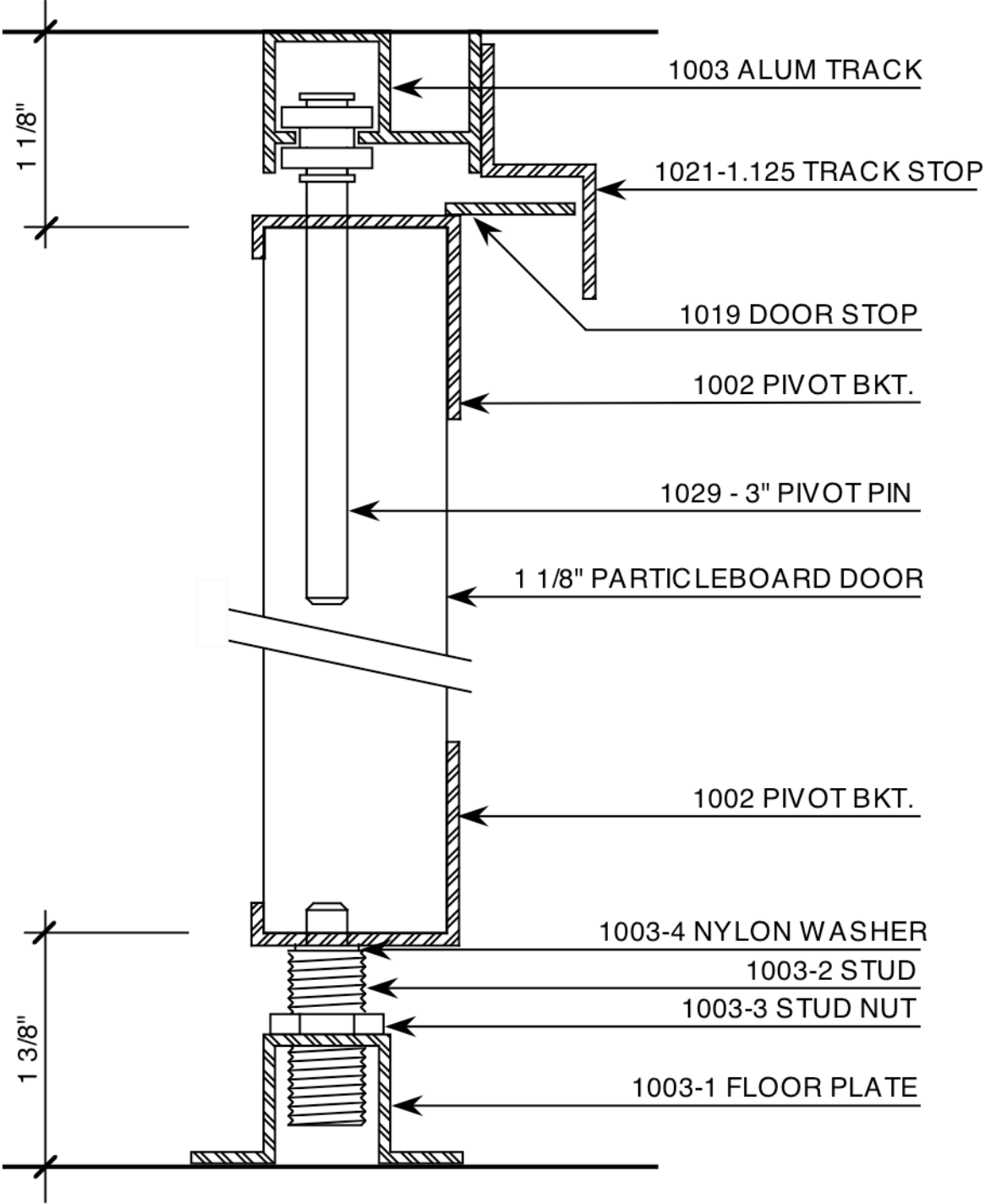
TYPICAL SECTION @ 1 1/8" BIFOLD DOOR
