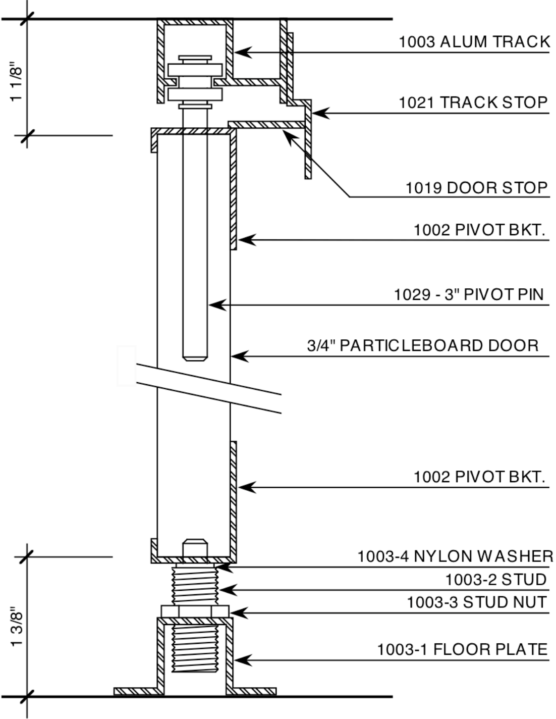
TYPICAL SECTION @ 3/4" BIFOLD
