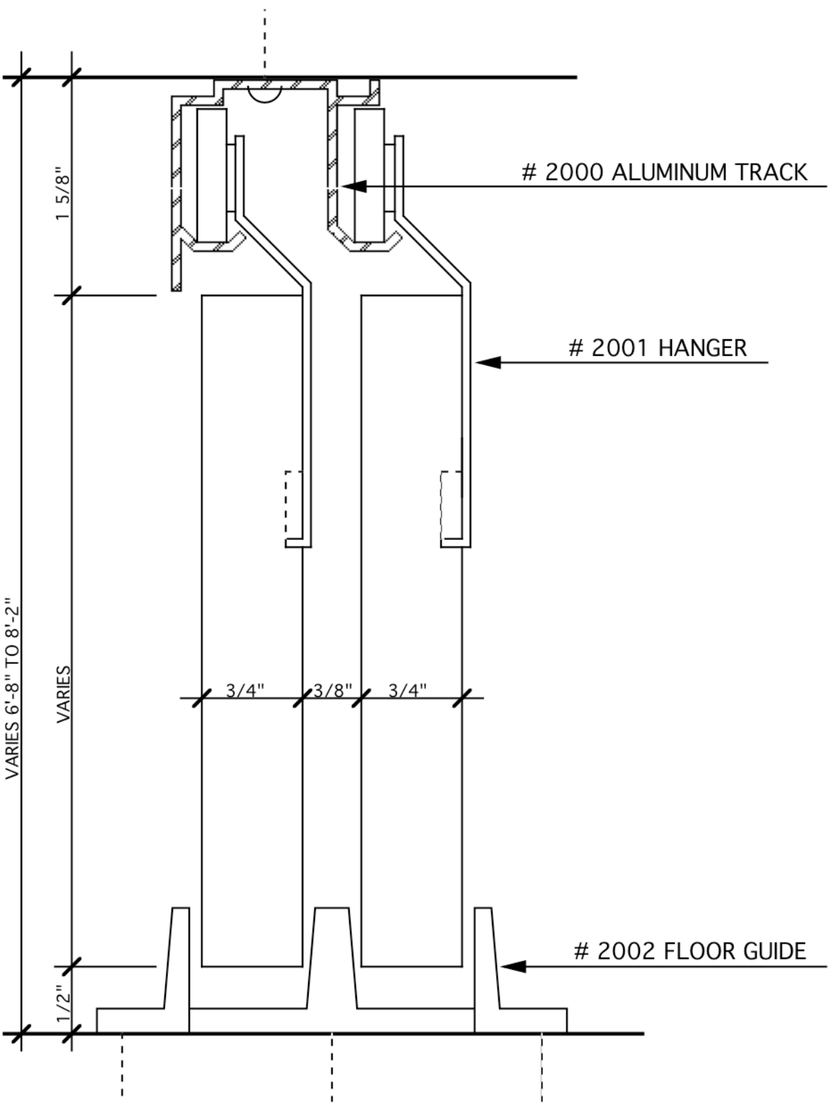
TYPICAL SECTION @ BI-PASS DOOR
