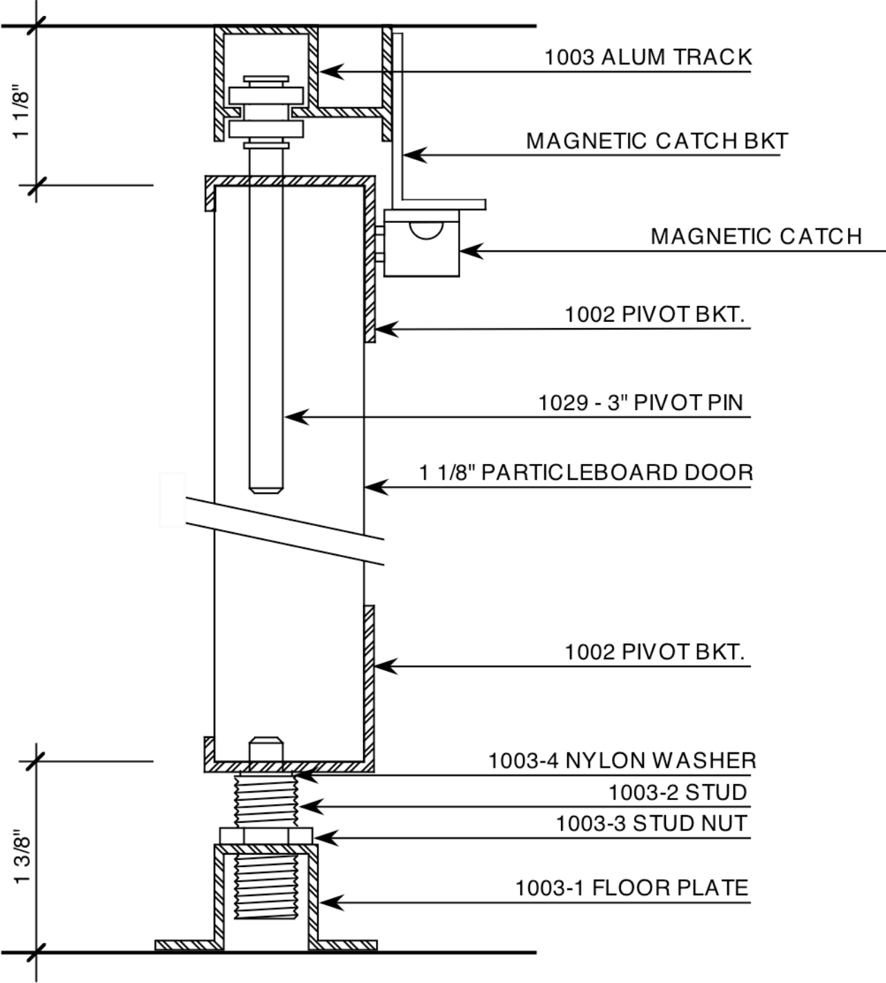
TYPICAL SECTION @ 1 1/8" PIVOT
