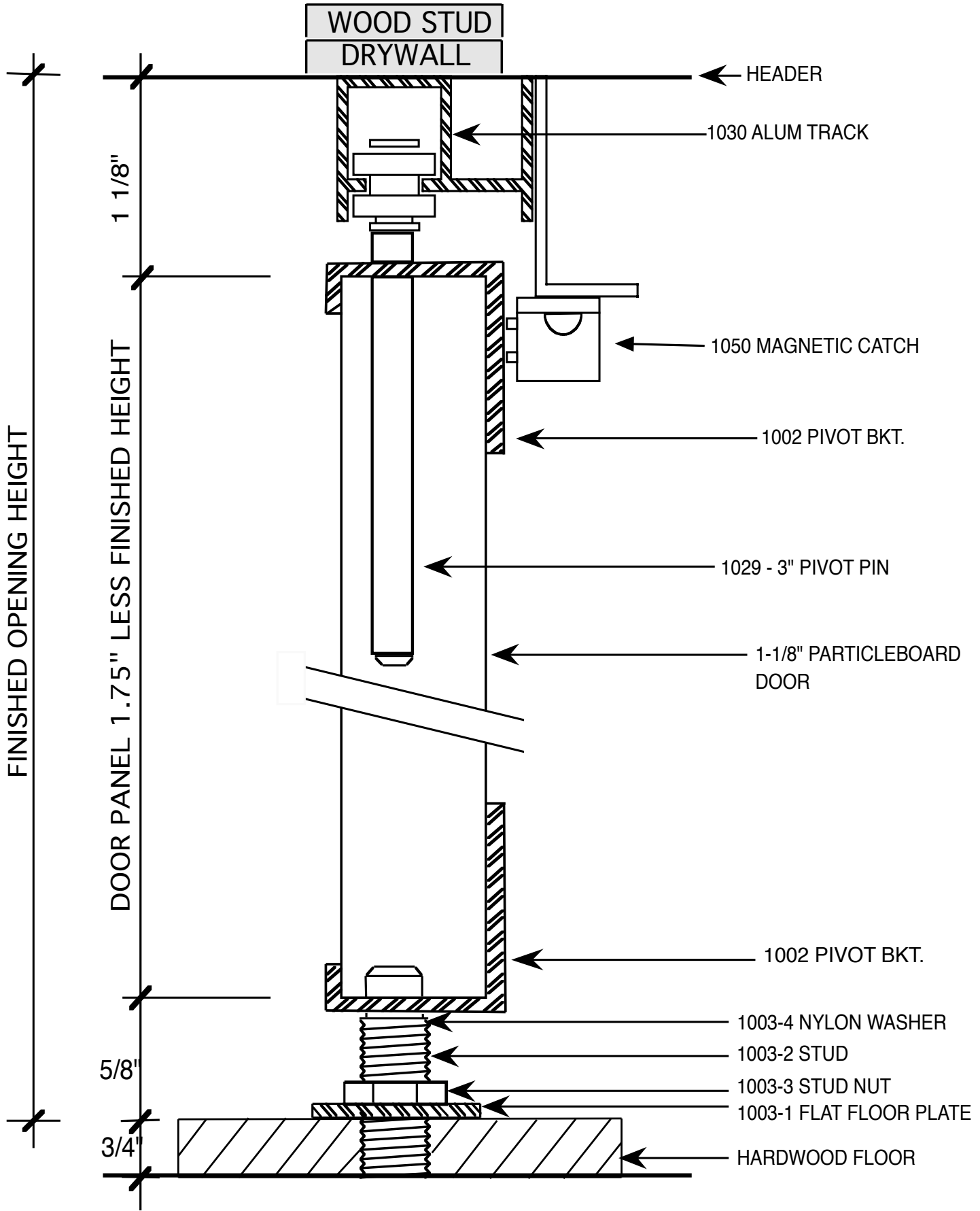
TYPICAL SECTION @ 1-1/8" PIVOT DOOR THIS FLOOR PLATE IS USED FOR HARDWOOD & TILE CONDITIONS
