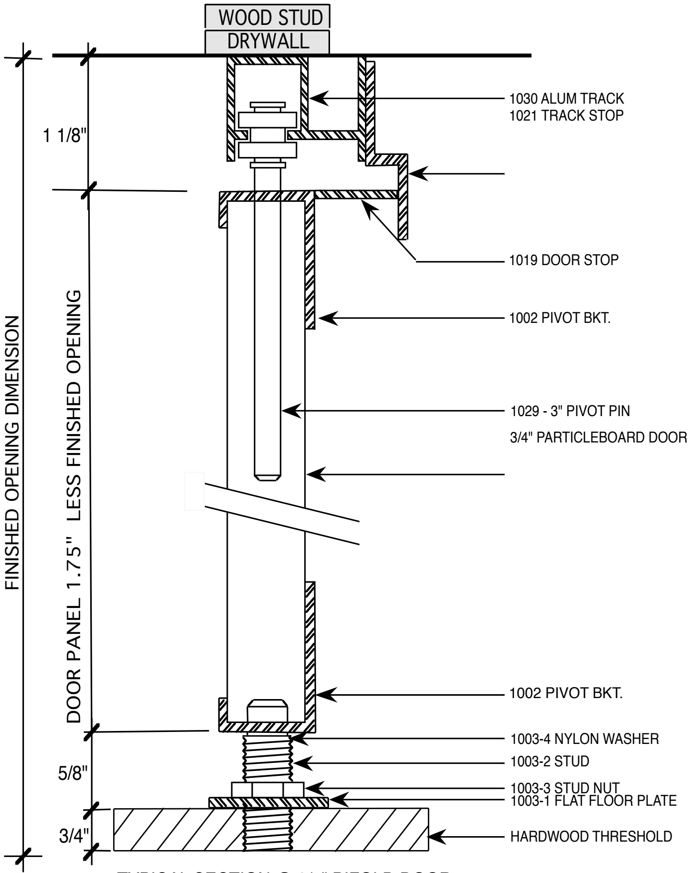
TYPICAL SECTION @ 3/4" BIFOLD DOOR THIS FLOOR PLATE IS USED FOR HARDWOOD & TILE CONDITIONS
