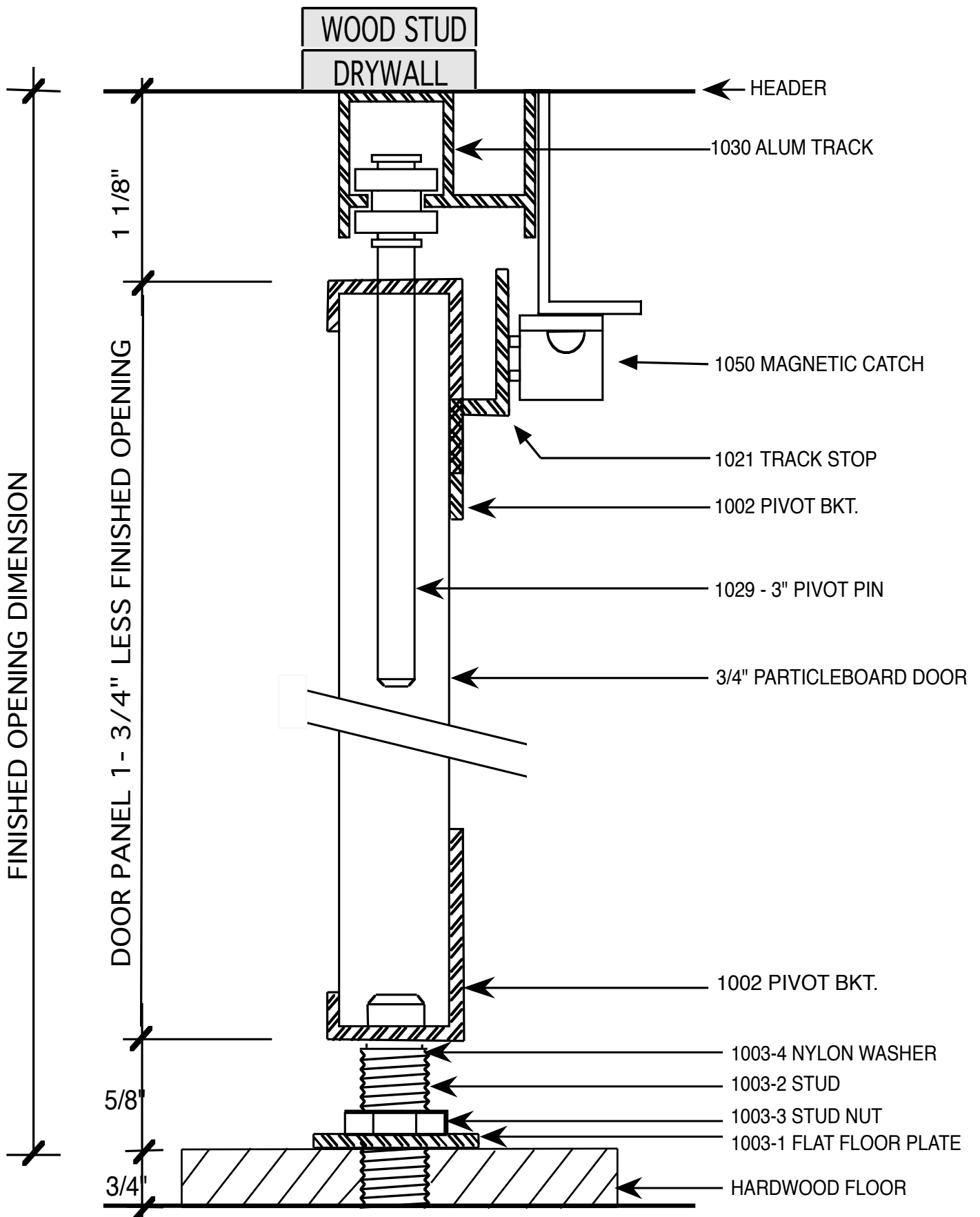
TYPICAL SECTION @ 3/4" PIVOT DOOR THIS FLOOR PLATE IS USED FOR HARDWOOD & TILE CONDITIONS
