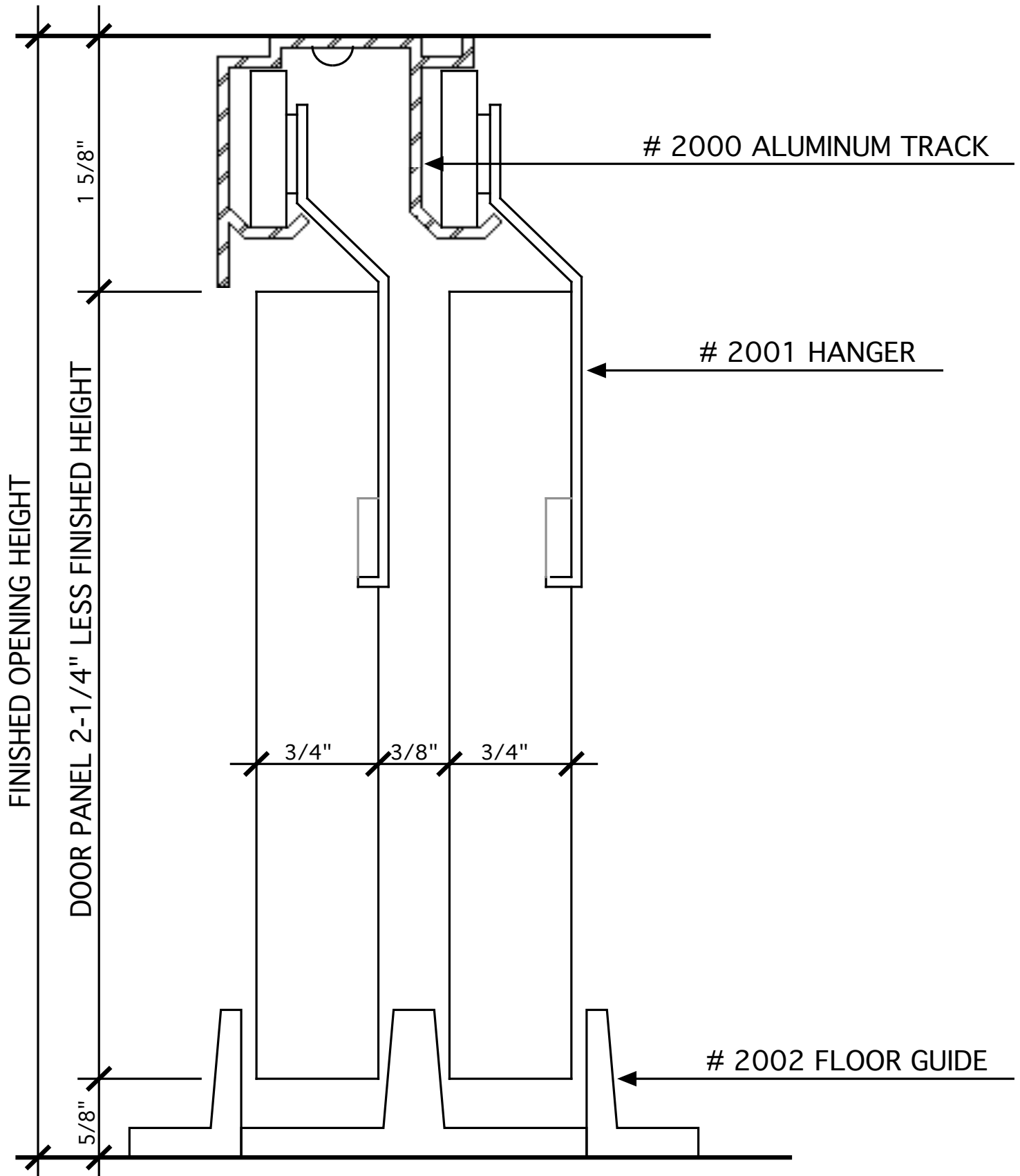
TYPICAL SECTION @ BI-PASS DOOR
