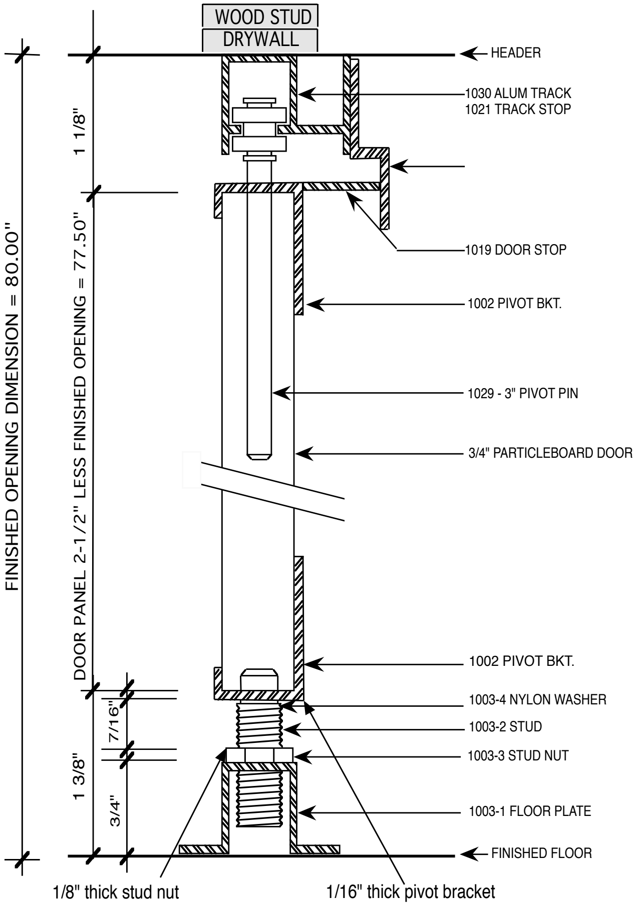
TYPICAL SECTION @ 3/4" BIFOLD DOOR
